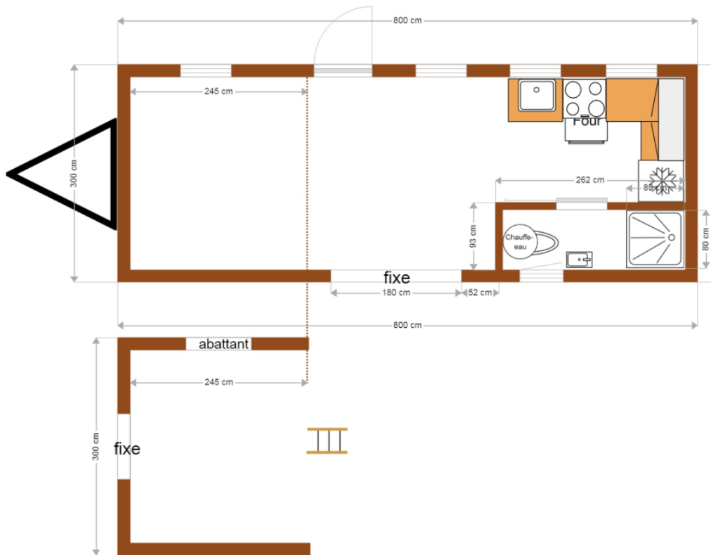
Plan L8003 size 8x3 m
