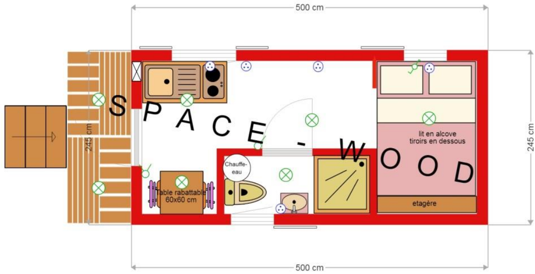
Plan L5001 size 5.90x2.45 m
