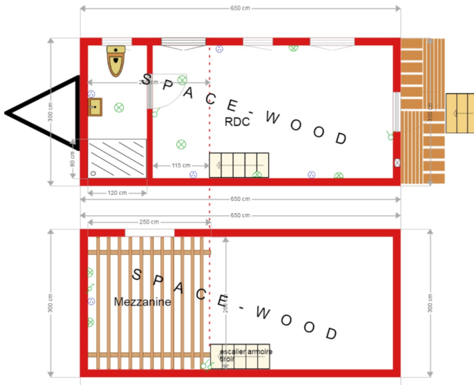
Plan L6501 size 7.40x3 m
